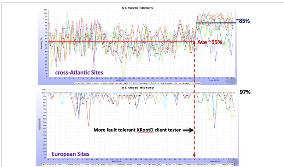
Figure 44. ALICE storage tests results for cross-Atlantic sites and those in Europe. Results indicated a network problem non-local to the grid sites instead of a local grid storage problem as originally thought.
