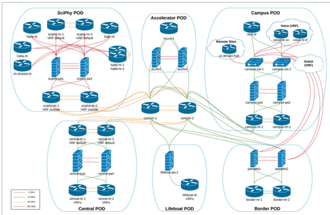
Figure 10. JLab layer 3 design.
