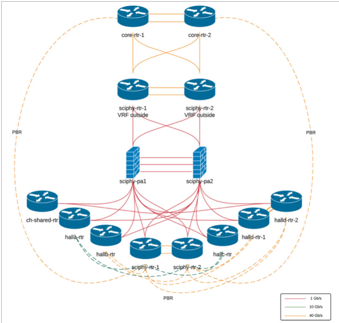
Figure 11. JLab Scientific Computing Network.
